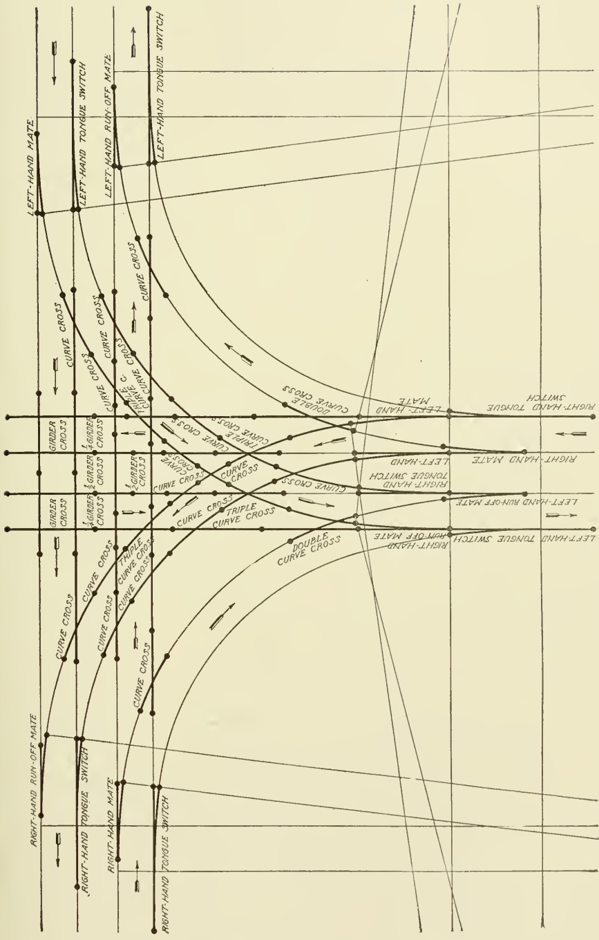
Fig. 238. Double Track Crossing with Connecting Curves
